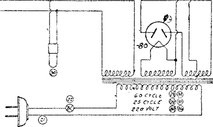
137 CHASSIS ASSEMBLY WIRING DIAGRAM
